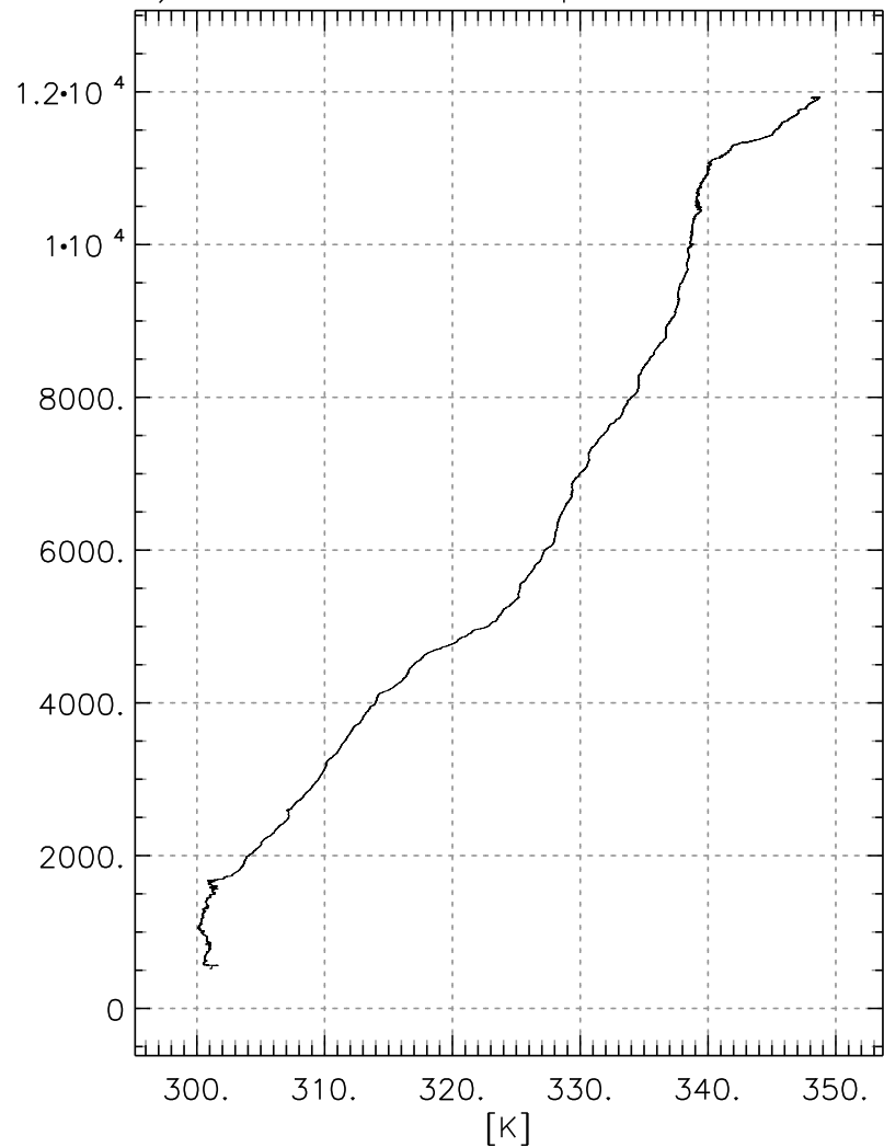
Potential Temperature
