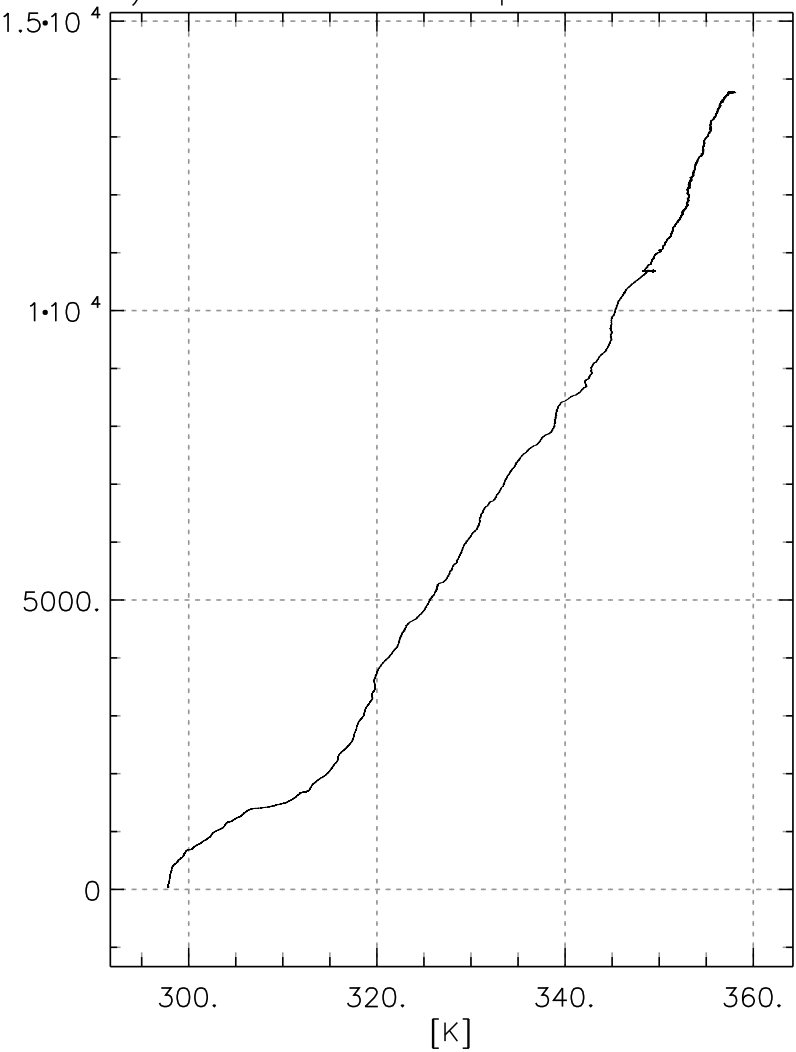
Potential Temperature
