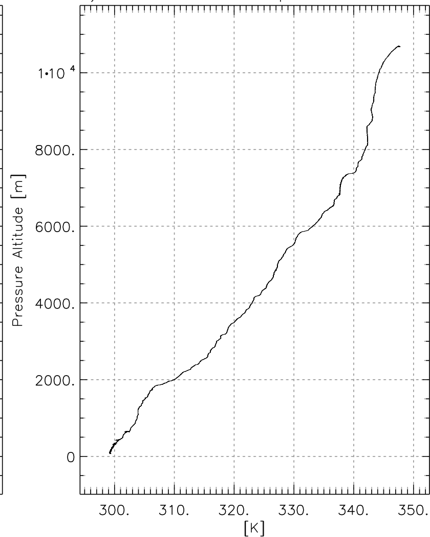
Potential Temperature
