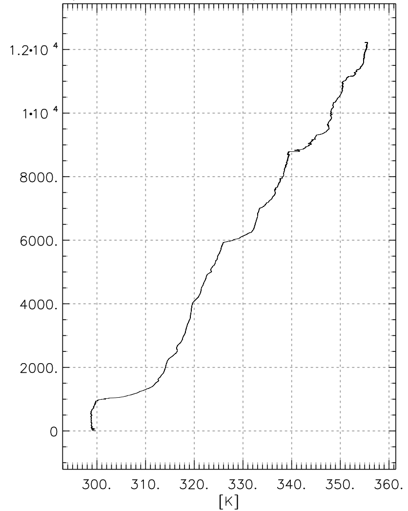
Potential Temperature
