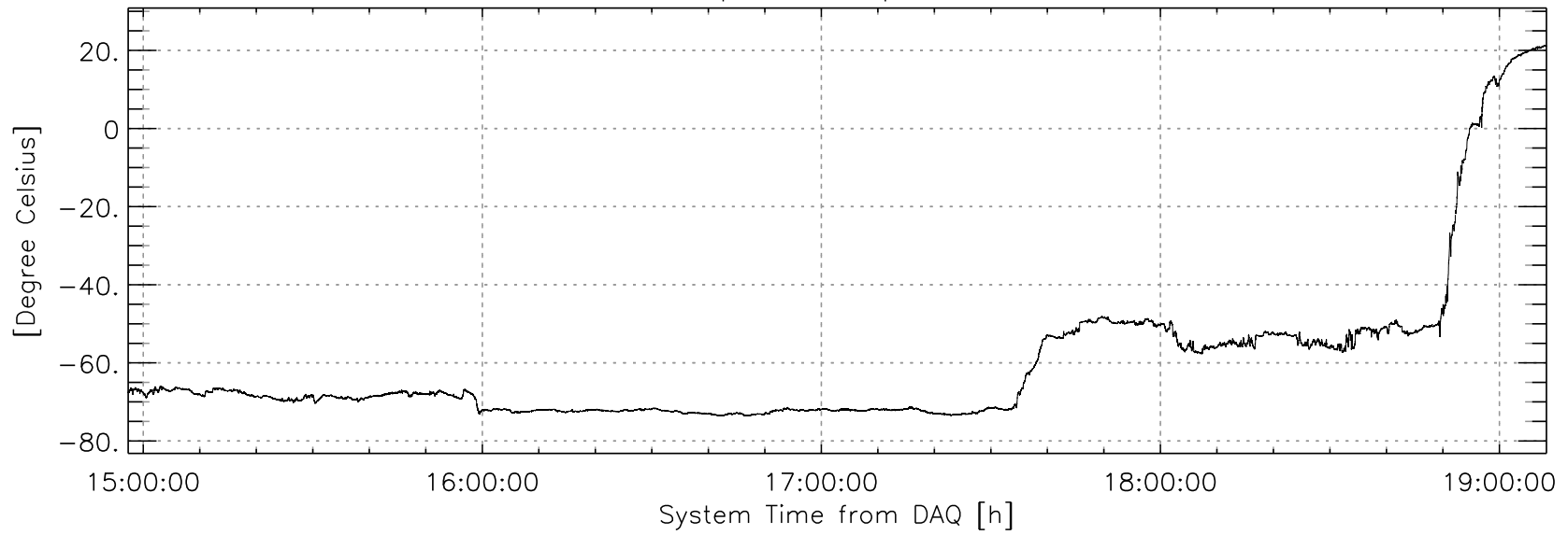
Dewpoint Temperature
