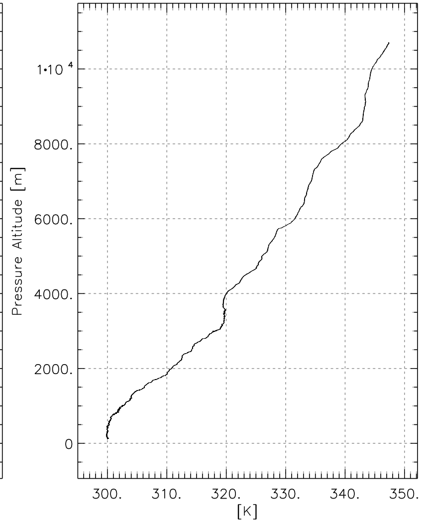
Potential Temperature
