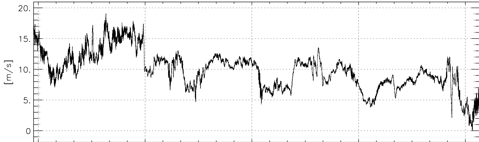
Horizontal Windspeed
