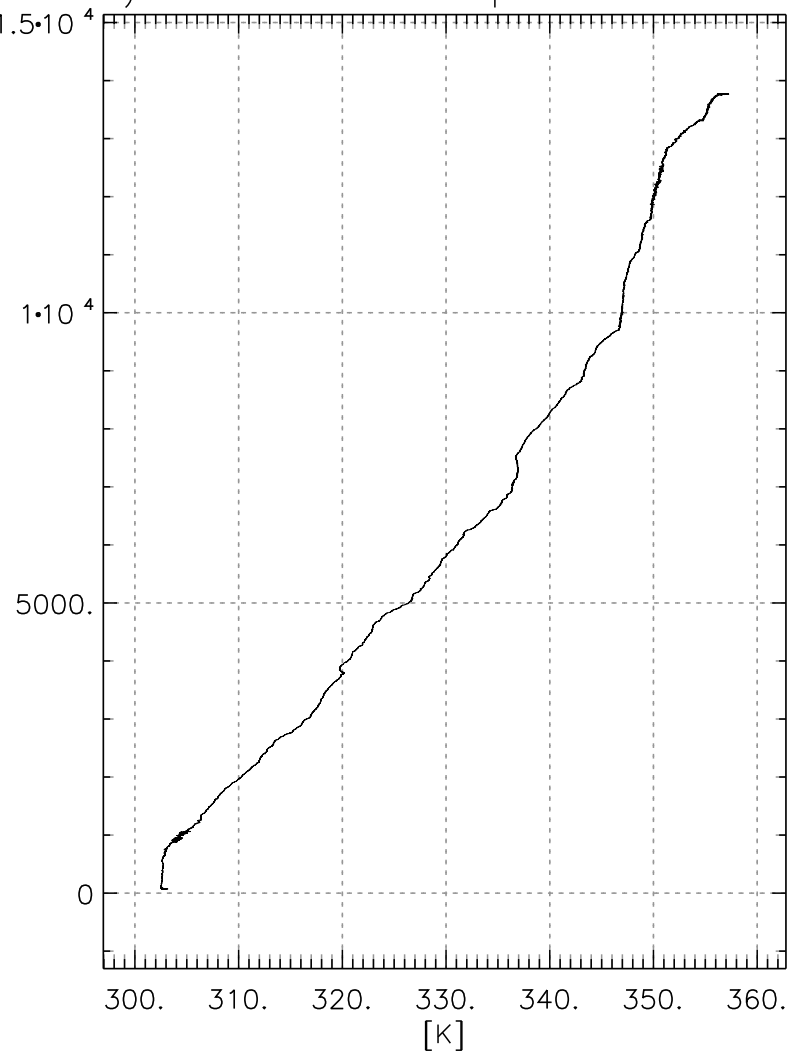
Potential Temperature
