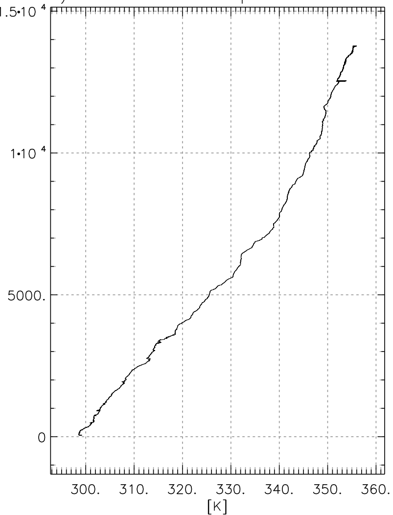
Potential Temperature
