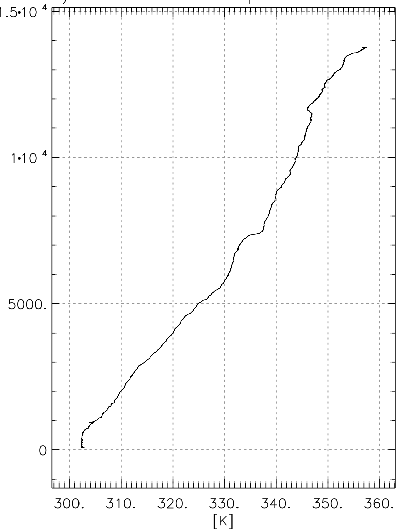
Potential Temperature
