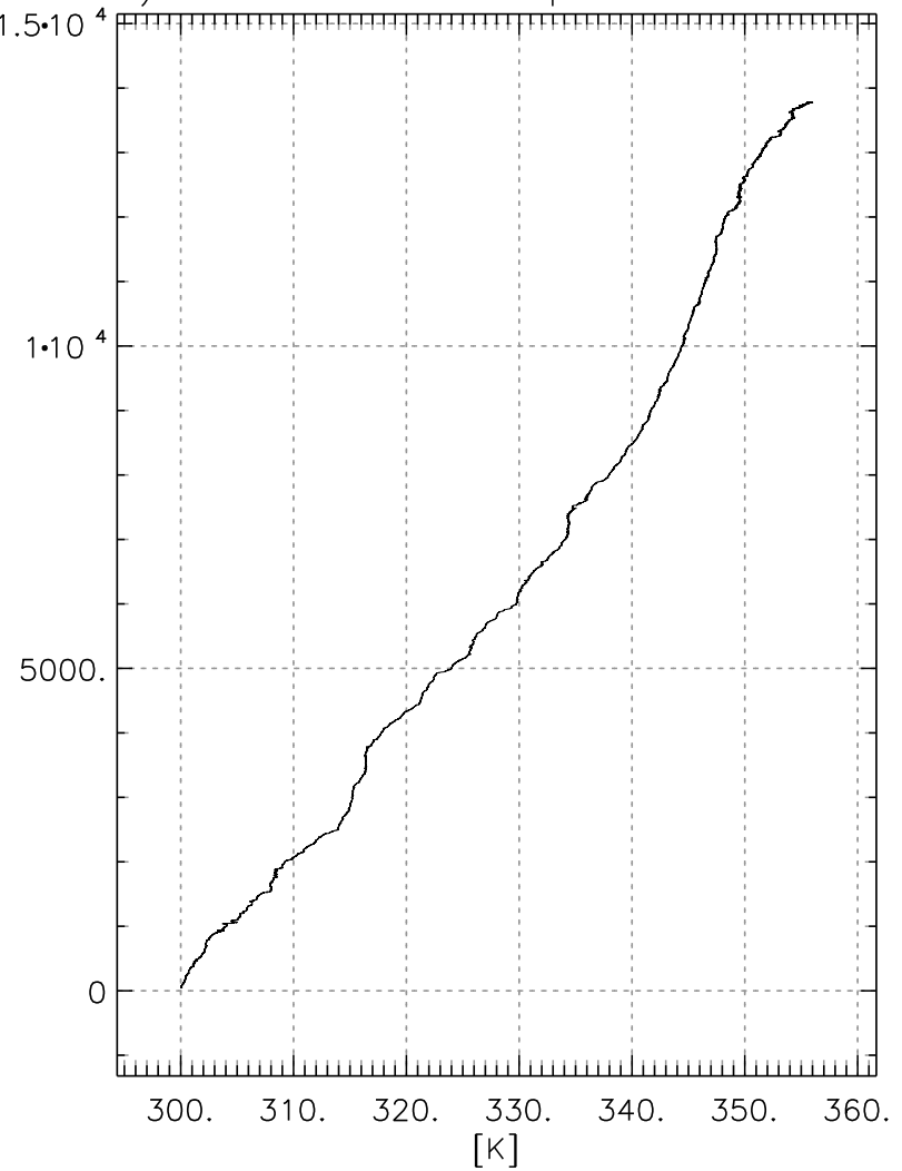
Potential Temperature
