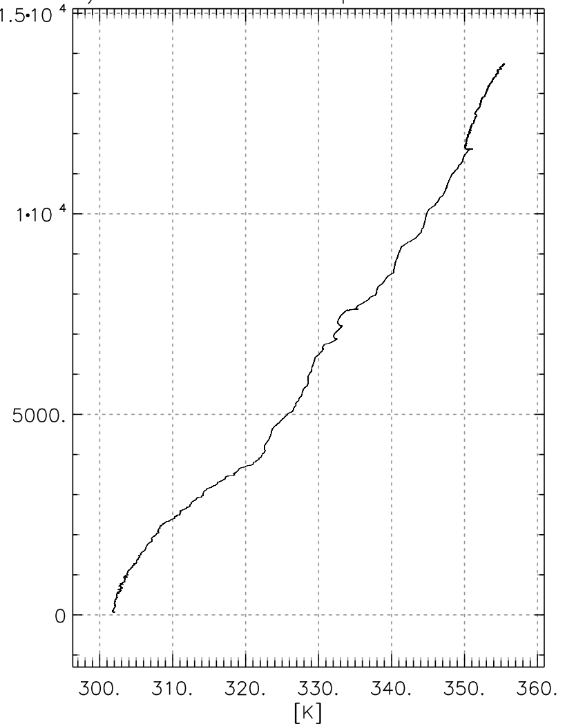
Potential Temperature
