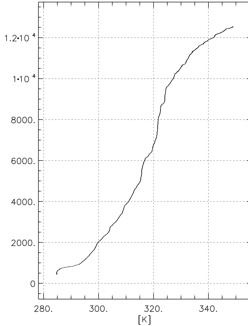
Potential Temperature
