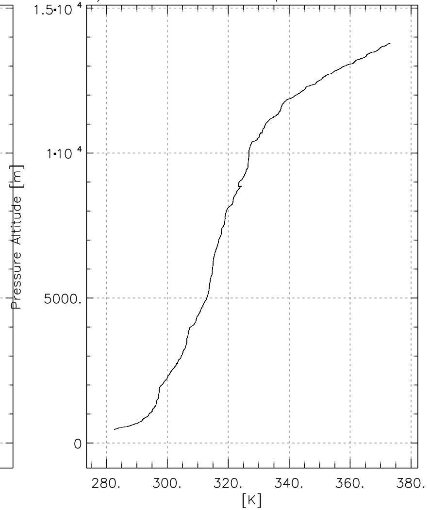
Potential Temperature
