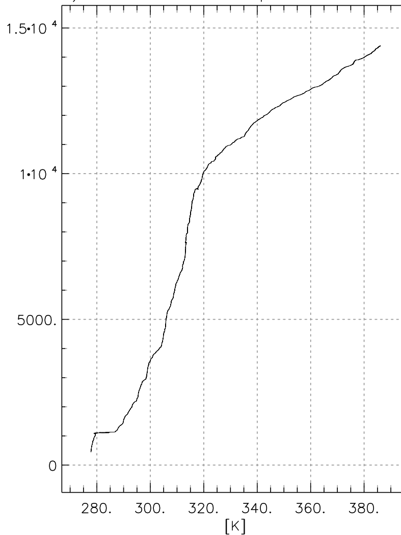
Potential Temperature
